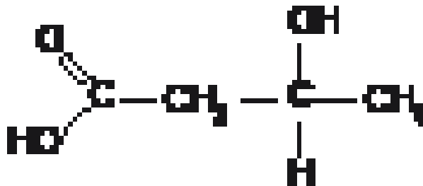
β-Hydroxybutyric acid
