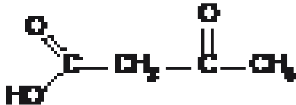
Acetoacetic acid
