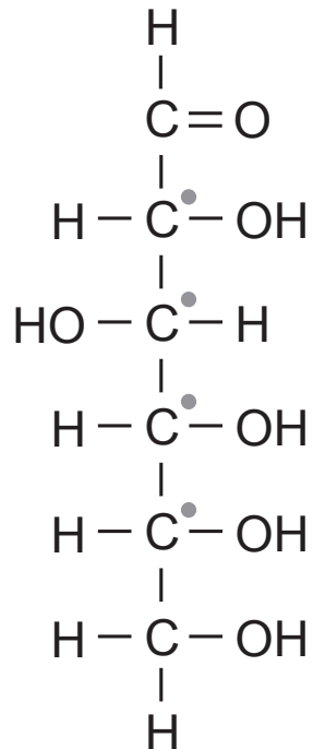
D-Glucose
