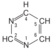
Pyrimidin
