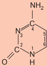
Cytosin (Cyt)
