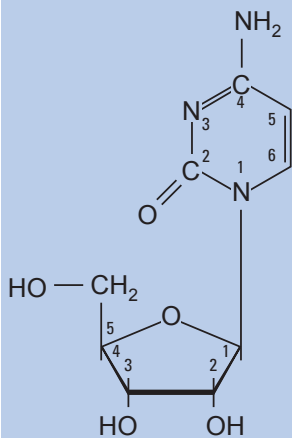
Cytidin (C)
