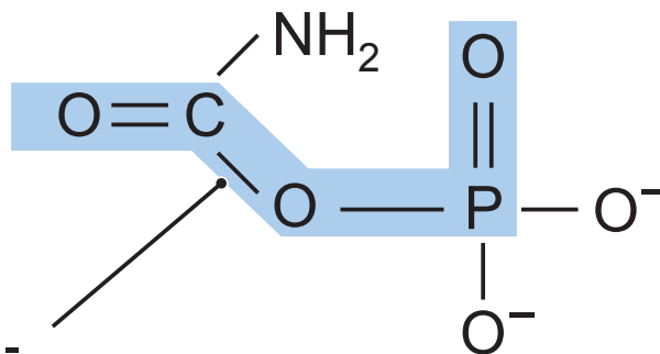
Carbamoylphosphat
