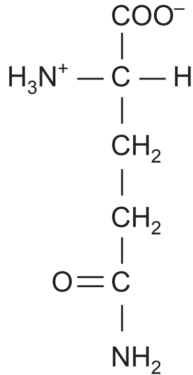
Glutamin
