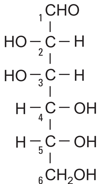
D-Mannose
