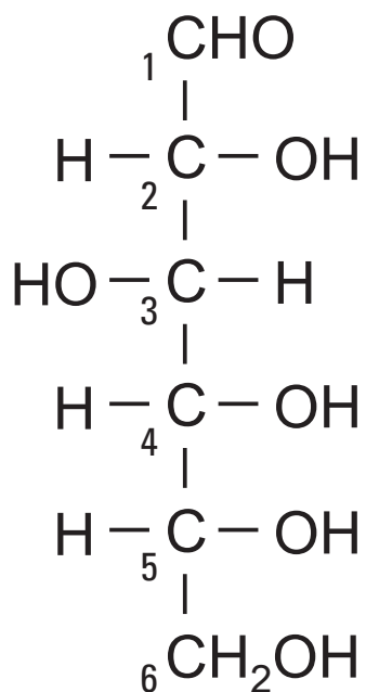
D-Glucose
