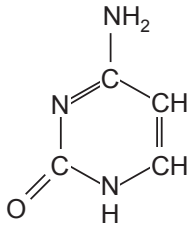
Cytosin (Cyt)
