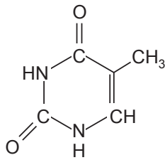
Thymin (Thy)
