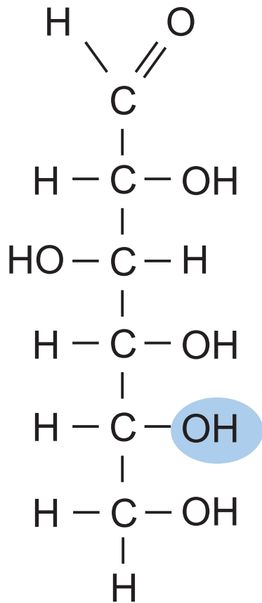
D-Glucose
