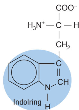
Tryptophan (Trp)*
