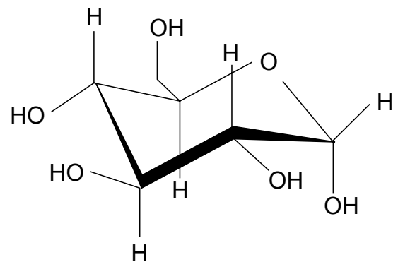
\alpha -D-Glucose
