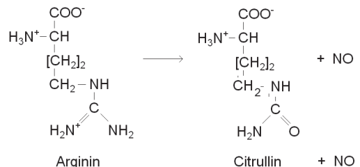
Abb. 38: NO-Synthese
