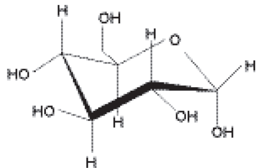
\alpha -D-Glucose
