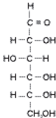
D-Glucose
