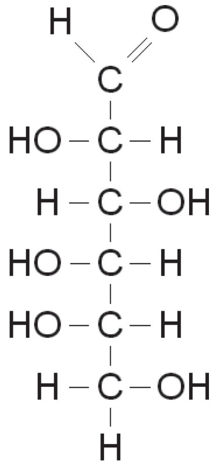
L-Glucose
