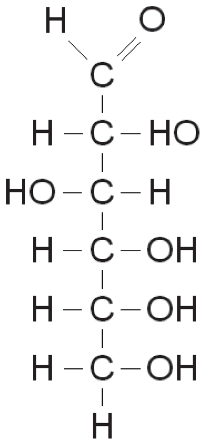
D-Glucose
