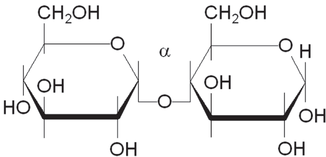
\alpha -Glucose (1,4)-Glucose
