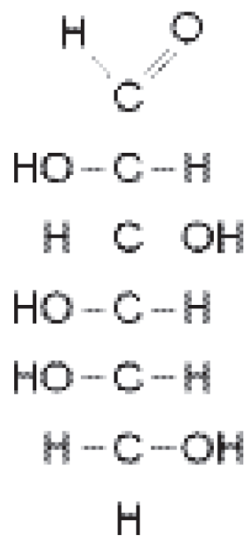
L-Glucose
