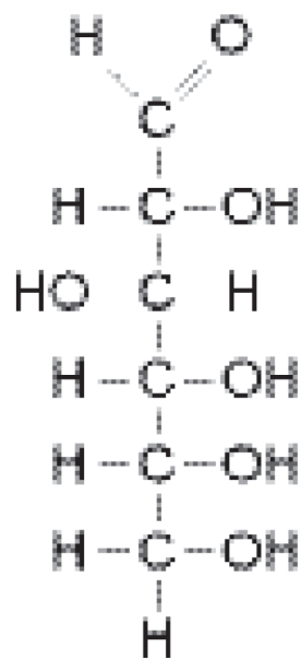
D-Glucose
