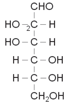
D-Mannose
