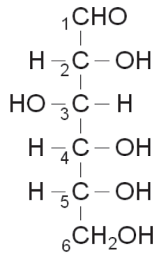
D-Glucose
