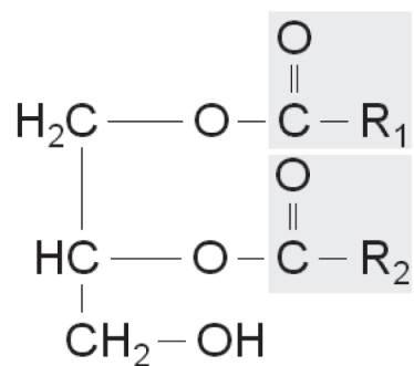
Diacylglycerid
