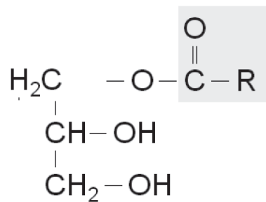
Monoacylglycerid
