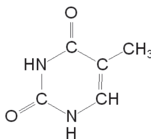
Thymin (Thy)
