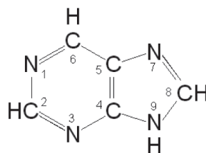
Purin
