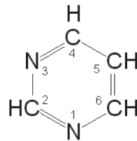
Pyrimidin
