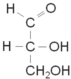
D - Glycerinaldehyd
