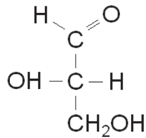
L - Glycerinaldehyd
