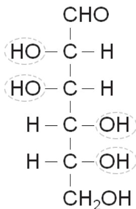
D - Mannose
