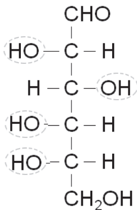
L - Glucose
