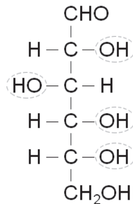
D - Glucose
