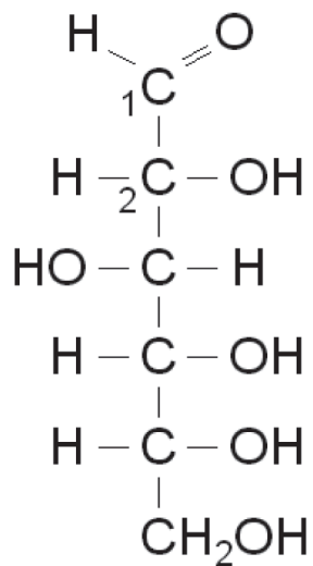
D-Glucose
