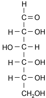
D-Glucose
