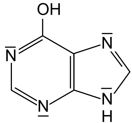
Enolform
