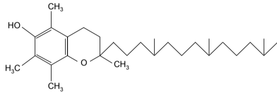
\alpha -Tocopherol
