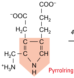
Porpho- bilinogen
