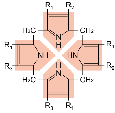
Uroporphyrinogen
