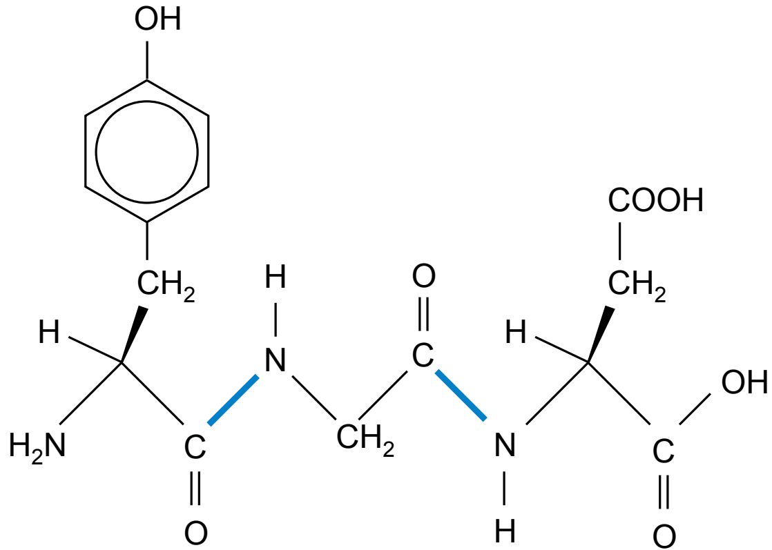
Tripeptid
