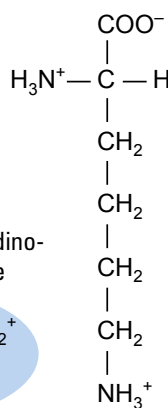
Lysin (Lys)*
