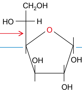
Furanose
