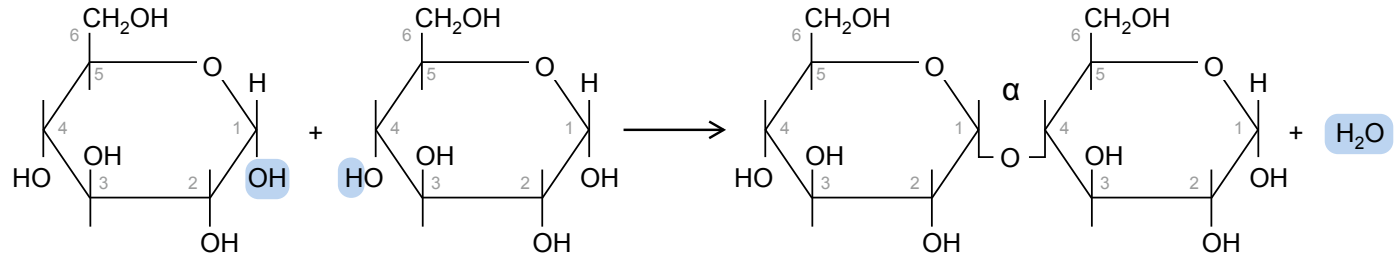
\alpha -D-Glucose
