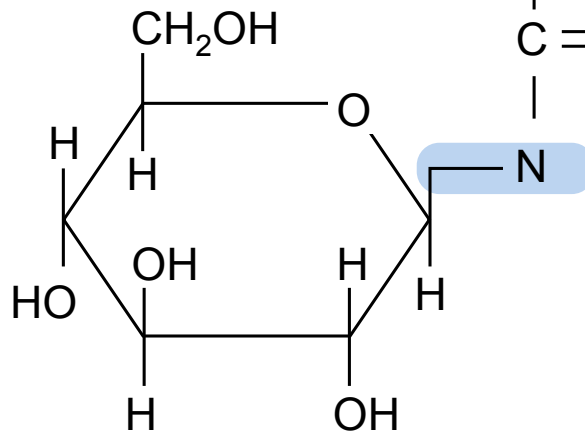
D-Glucose
