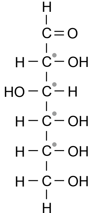
D-Glucose
