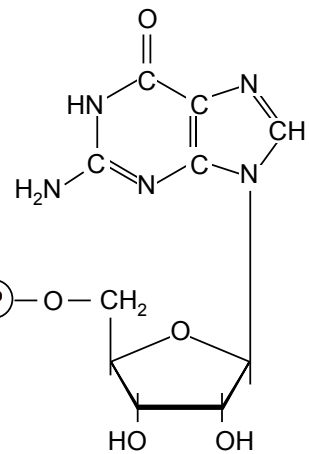
Guanosinmonophosphat GMP
