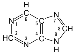
Purin
