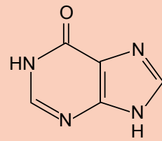
Hypoxanthin (Hyp)
