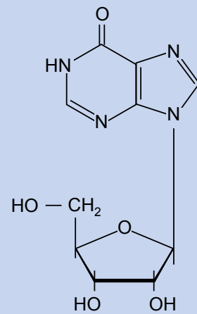
Inosin (I)
