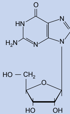
Guanosin (G)
