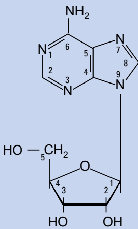
Adenosin (A)
