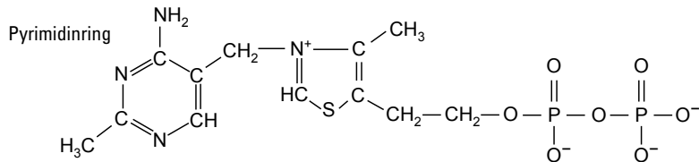
Thiaminpyrophosphat
