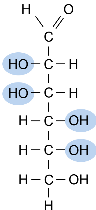
D-Mannose
