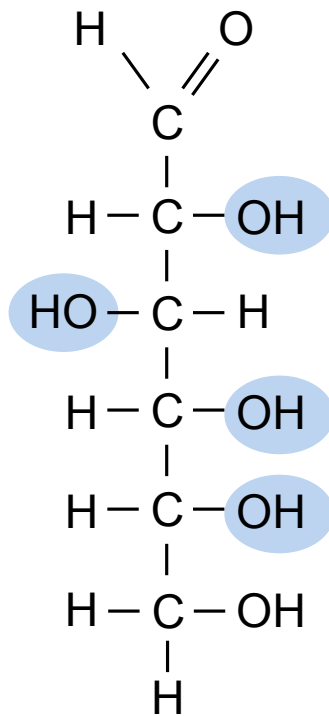
D-Glucose
