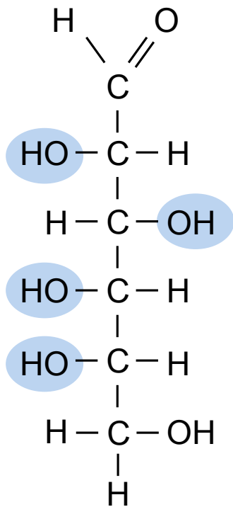
L-Glucose
