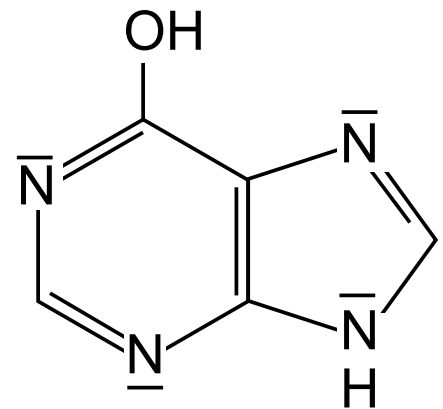
Enolform
