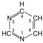
Pyrimidin
