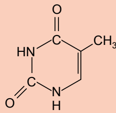
Thymin (Thy)
