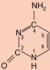
Cytosin (Cyt)
