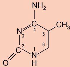
5-Methylcytosin
