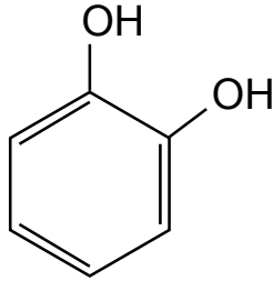
Katechol (1,2-Dihydroxybenzol)
