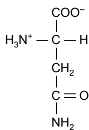
Asparagin (Asn)
