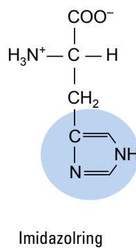
Histidin (His)
