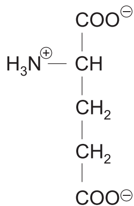
Glutamat
