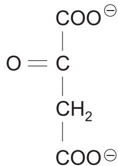
Oxalacetat
