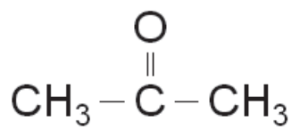
Aceton
