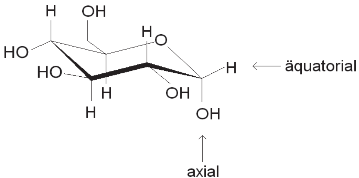
\alpha -D-Glucose
