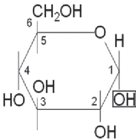
\alpha -D-Glucose
