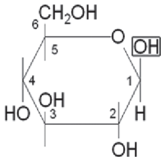
\beta -D-Glucose
