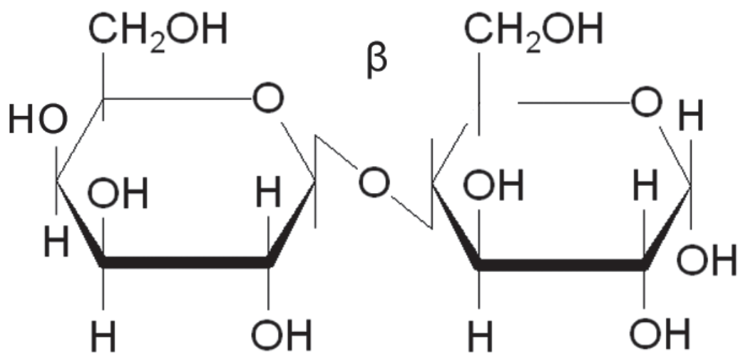
\beta -Galaktose (1,4)-Glucose
