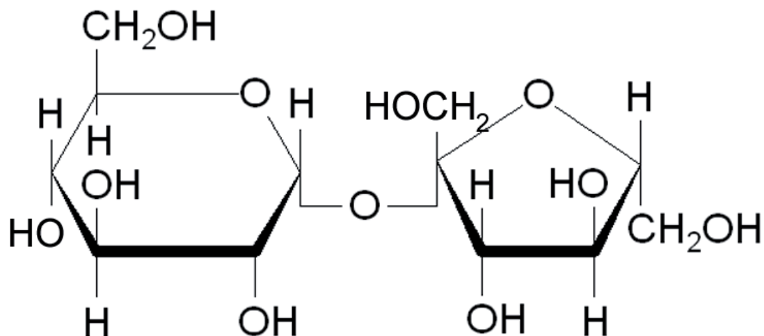
\alpha -Glucose (1,2)- \beta -Fructose
