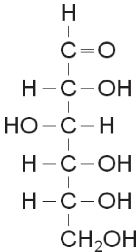
D-Glucose
