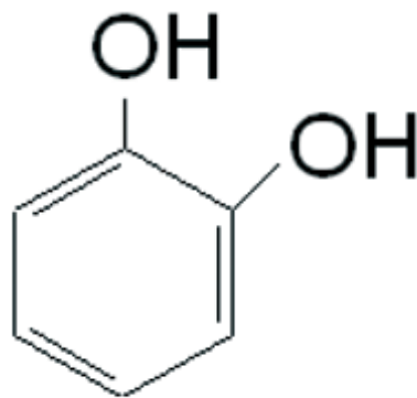
Katechol (= 1,2-Dihydroxybenzol)
