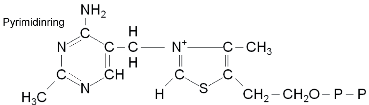
Thiaminpyrophosphat
