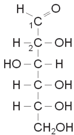
D-Glucose
