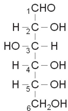
D-Glucose
