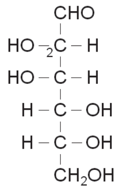
D-Mannose
