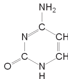
Cytosin (Cyt)
