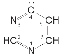
Pyrimidin
