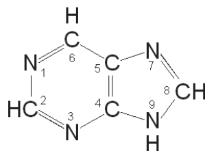
Purin
