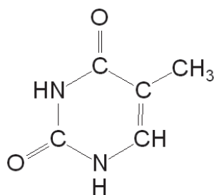
Thymin (Thy)
